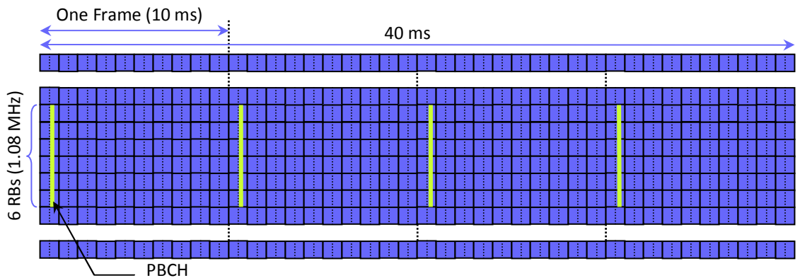
FIGURE 10 PBCH STRUCTURE.
