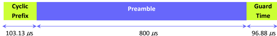
FIGURE 14 RANDOM ACCESS PREAMBLE.
